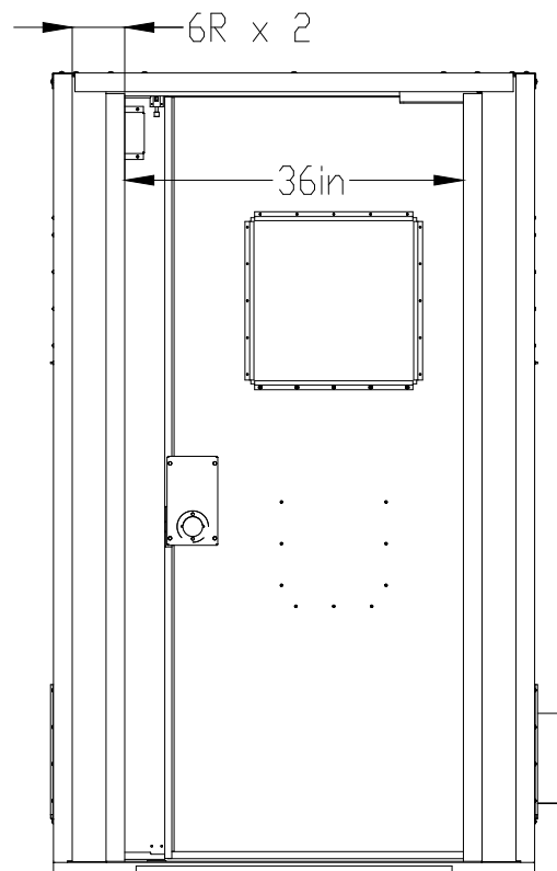
48" AnteRoom with 6RR & 6LR reducers to fit 36" Door
